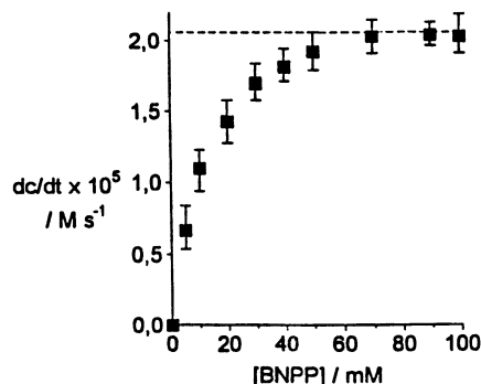
Fig. 10. Saturation kinetics for the hydrolysis of BNPP by (L¹)Cu (5 mM). Reaction conditions: ethanol–water 19:1, 20°C, pH 6.6.
